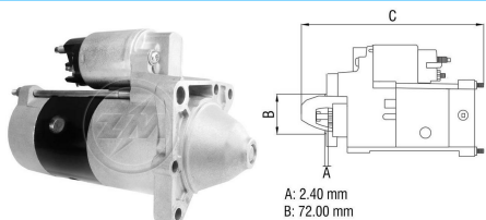
Starter Drive
