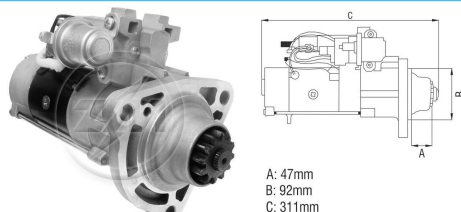
Starter Drive
