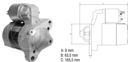
Starter Drive
