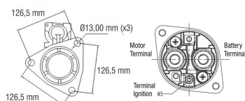
Drive Housing
