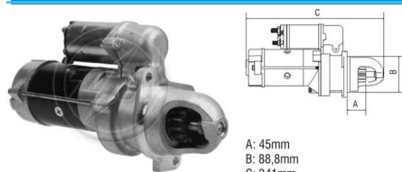
Starter Drive
