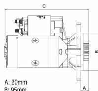
Starter Solenoid
