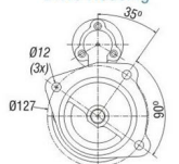
Drive Housing
