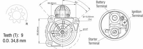
Starter Drive
