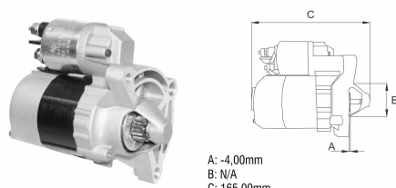
Starter Drive
