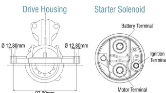
Drive Housing
