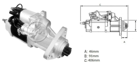
Starter Drive
