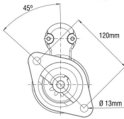
Drive Housing
