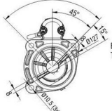
Drive Housing
