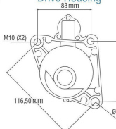
Drive Housing
