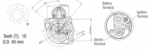
Starter Drive
