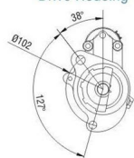
Drive Housing
