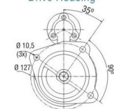
Drive Housing
