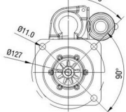
Drive Housing
