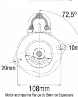
Drive Housing
