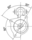
Drive Housing
