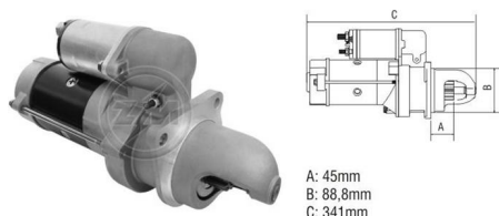
Starter Drive
