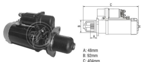
Starter Drive
