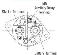
Starter Solenoid
