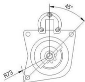
Drive Housing
