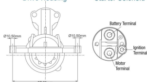
Drive Housing
