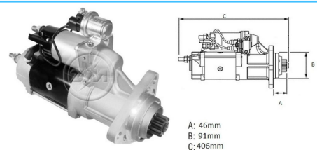
Starter Drive
