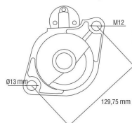
Drive Housing
