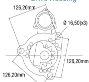
Drive Housing
