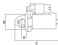
Starter Solenoid
