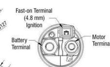
Starter Solenoid
