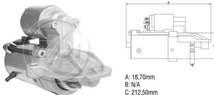
Starter Drive
