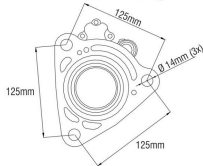
Drive Housing
