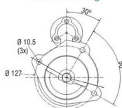
Drive Housing
