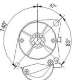
Drive Housing
