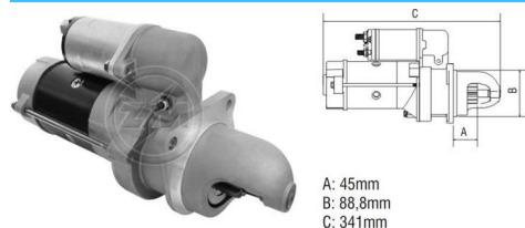
Starter Drive
