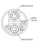
Starter Solenoid
