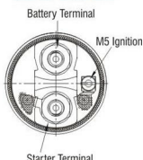
Starter Solenoid
