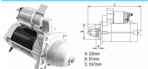
Starter Drive
