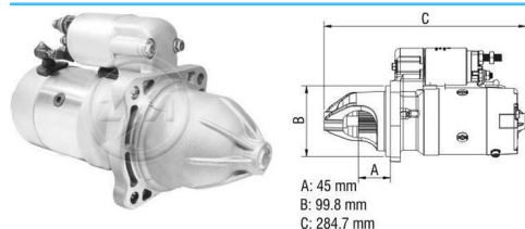
Starter Drive
