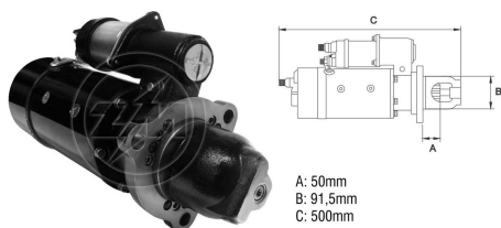
Starter Drive
