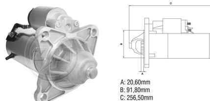
Starter Drive
