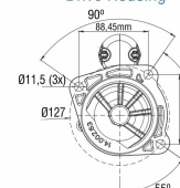
Drive Housing
