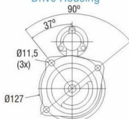
Drive Housing
