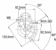
Drive Housing
