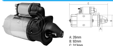
Starter Drive
