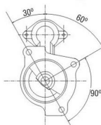
Drive Housing
