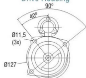
Drive Housing
