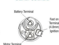
Starter Solenoid
