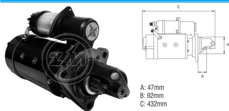
Starter Drive
