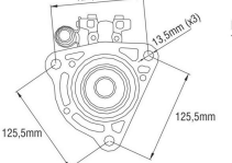
Drive Housing
