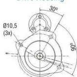
Drive Housing
