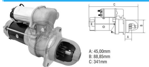
Starter Drive
