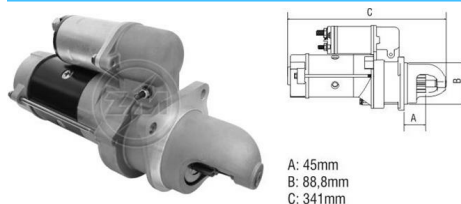
Starter Drive
