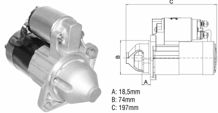
Starter Drive
