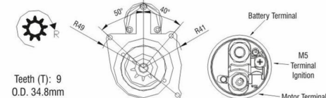
Starter Drive
