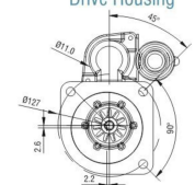
Drive Housing
