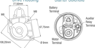
Drive Housing
