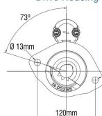
Drive Housing
