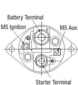
Starter Solenoid
