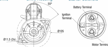
Starter Drive
