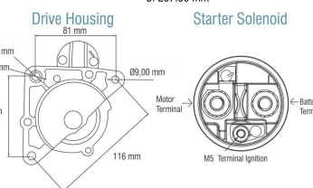
Starter Drive
