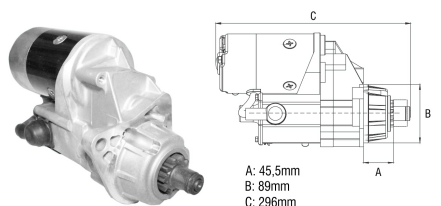
Starter Drive
