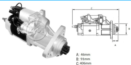
Starter Drive
