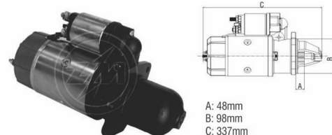
Starter Drive
