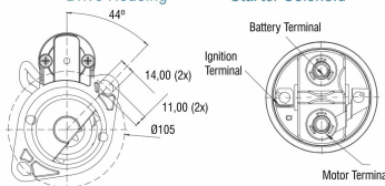
Drive Housing
