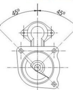
Drive Housing
