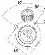
Drive Housing
