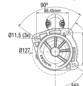
Drive Housing
