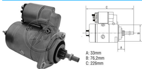
Starter Drive
