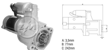
Starter Drive
