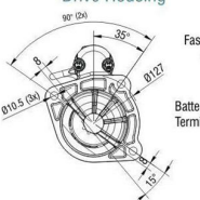
Drive Housing
