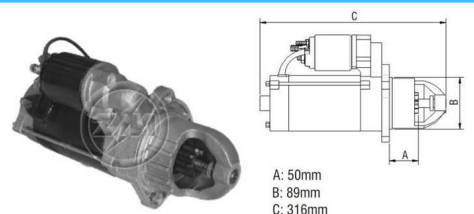
Starter Drive
