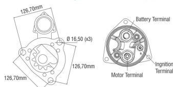
Drive Housing
