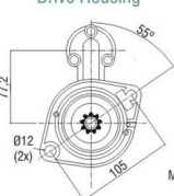
Drive Housing
