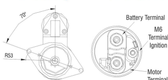
Drive Housing
