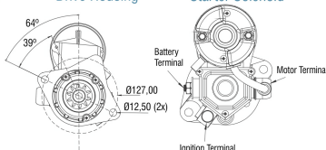
Drive Housing
