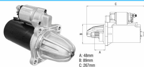
Starter Drive
