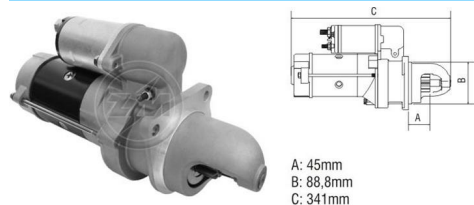
Starter Drive
