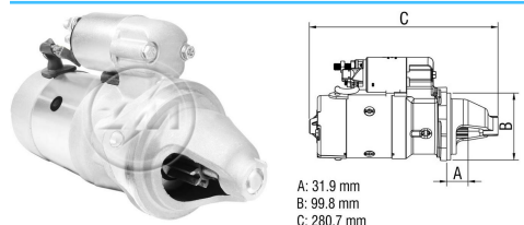
Starter Drive
