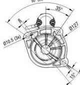
Drive Housing
