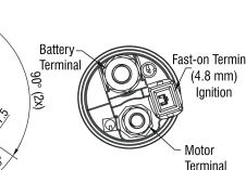
Starter Solenoid
