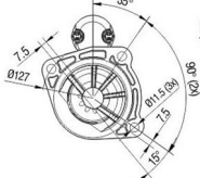
Drive Housing
