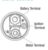
Starter Solenoid
