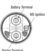
Starter Solenoid
