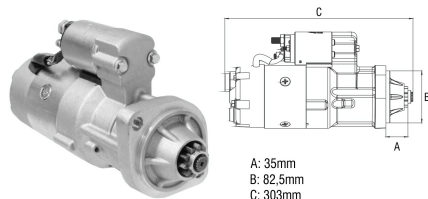
Starter Drive
