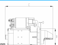
Starter Solenoid
