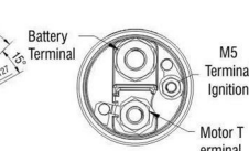
Starter Solenoid
