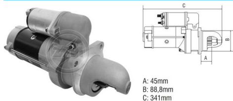
Starter Drive
