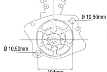
Drive Housing
